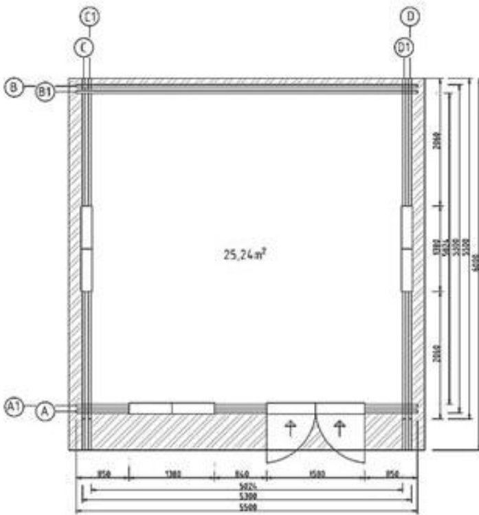
Ventina Twin-Wall 5.3x5.3 floor plan
