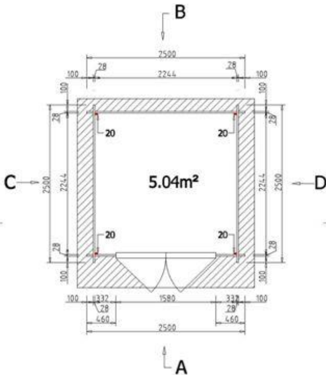
Bradnor floor plan
